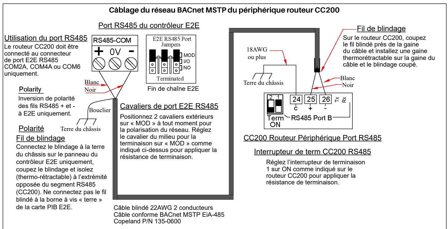
BACnet Router Device MS/TP Wiring
