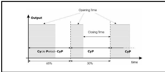
Figure 15-2 - Regulation Diagram
