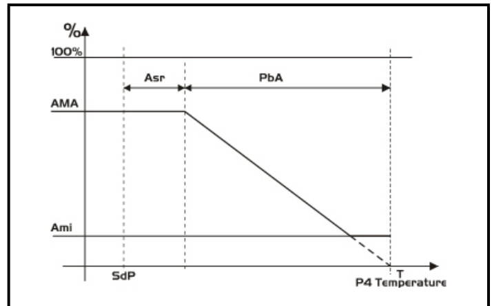
Figure 15-6 - Anti-Sweat Heaters
