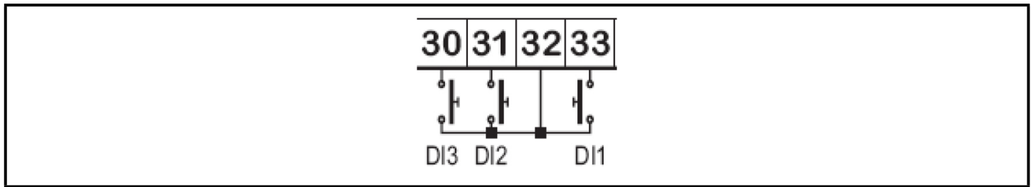
Figure 5-9 - Digital Inputs
