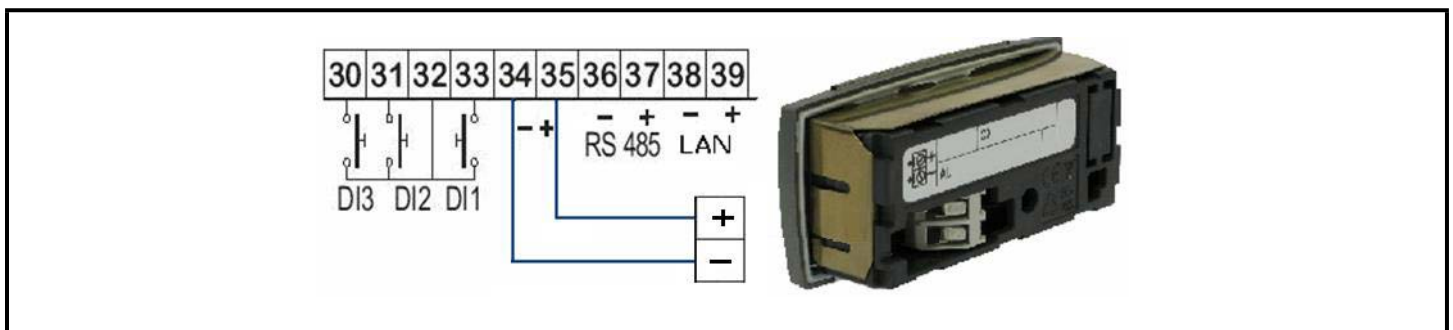
Figure 5-3 - Keyboard Display
