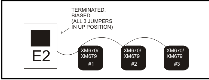
Figure 21-4 - MODBUS Networking
