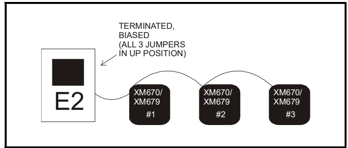
Figure 21-2 - MODBUS Networking
