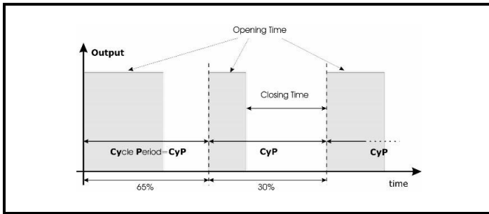
Figure 15-2 - Regulation Diagram
