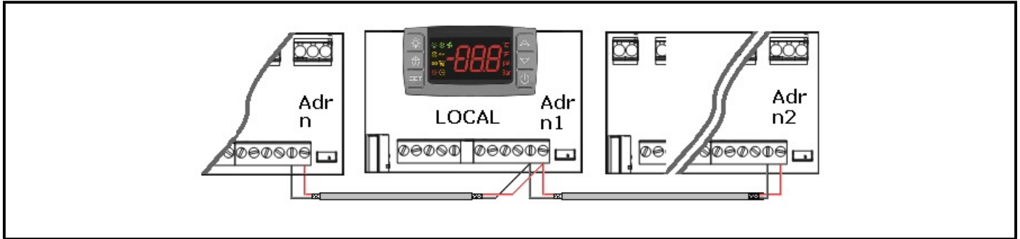
Figure 10-1 - LAN Connection
