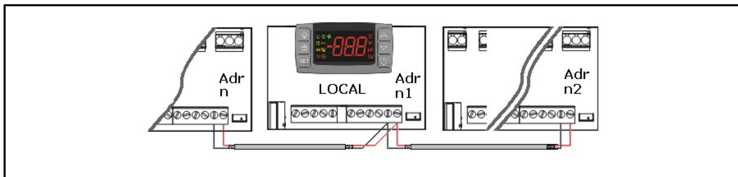
Figure 10-1 - LAN Connection
