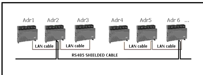
Figure 10-2 - Configuration Example
