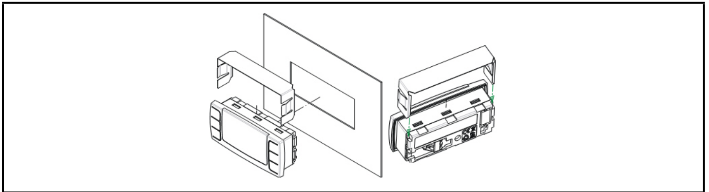
Figure 4-1 - CX660 Keyboard Installation and Mounting
