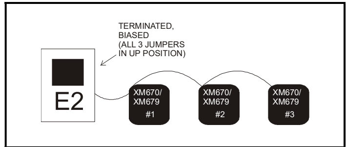
Figure 21-2 - MODBUS Networking
