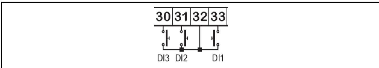
Figure 5-9 - Digital Inputs
