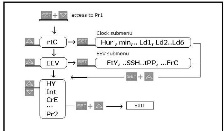
Figure 8-1 - General Structure
