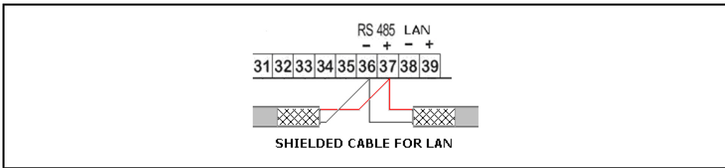
Figure 5-7 - Connecting the Monitoring System
