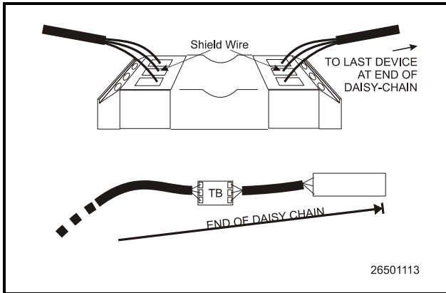
Figure 6-3 - MODBUS Termination Block (P/N 535-2711)
