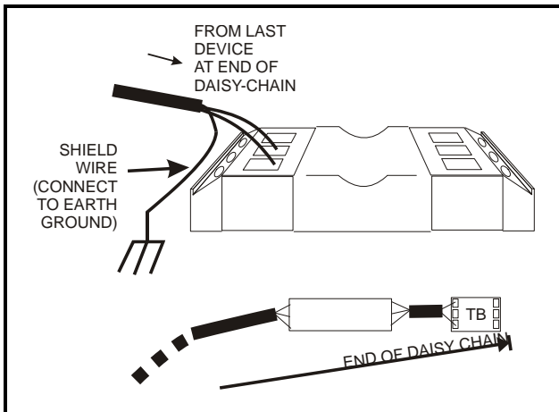
Figure 6-4 - MODBUS Term Block End-of-Chain Install
