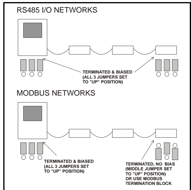
Figure 6-2 - I/O Network and MODBUS Termination and Biasing
