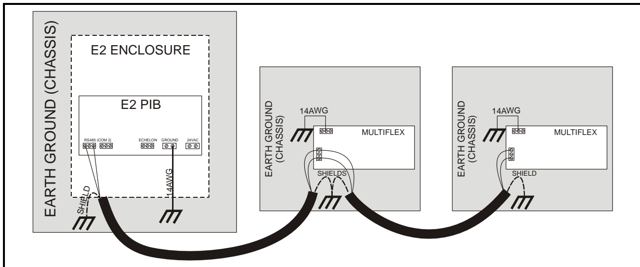
Figure 7-2 - RS485 Network Segment Grounding Practices (E2 and MultiFlex)
