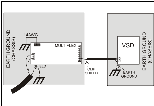
Figure 7-3 - MultiFlex and AO Cable Grounding
