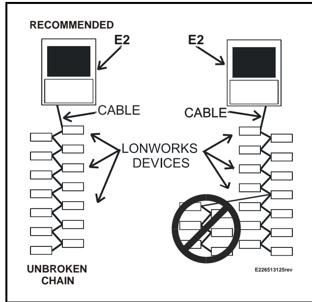
Figure 6-5 - Echelon Wiring - Subnets
