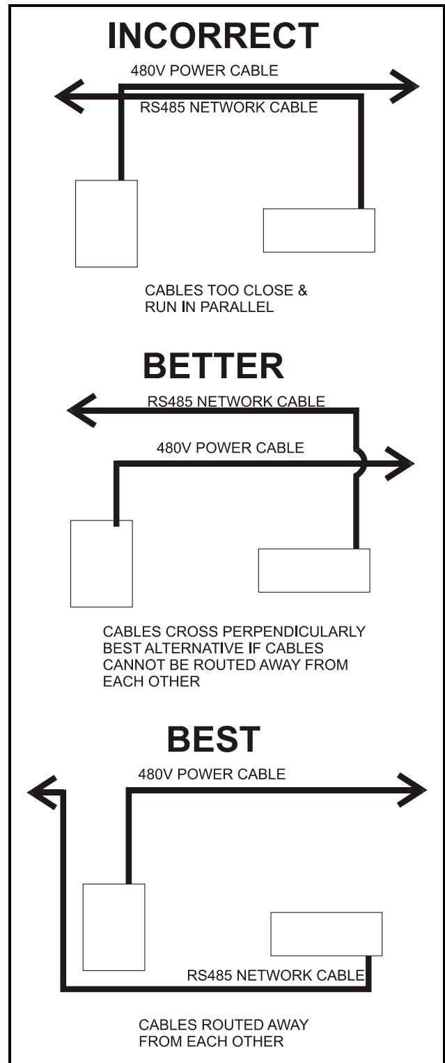
Figure 3-1 - Examples of Good & Bad Cable Routing
