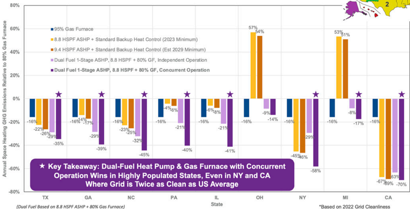
Figure 5: GHG emissions per residential home heating in states with the highest single-family homes relative to 80% gas furnace
