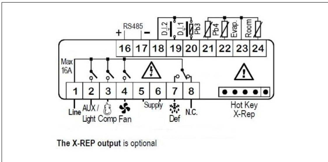
Figure 16-1 - XR75CX Connections
