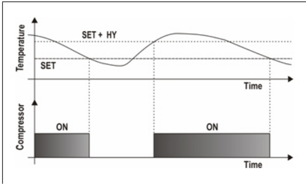
Figure 3-1 - Compressor Temperature Regulation
