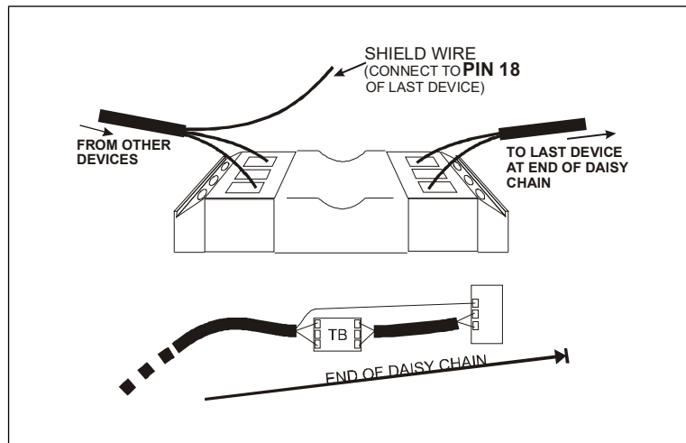
Figure 18-9 - MODBUS Termination Block (P/N 535-2711)
