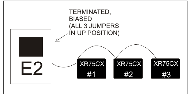
Figure 18-2 - MODBUS Networking
