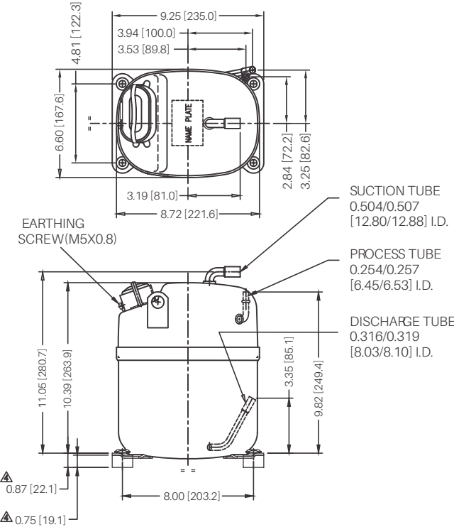
KCJ***CAL with suction tube
