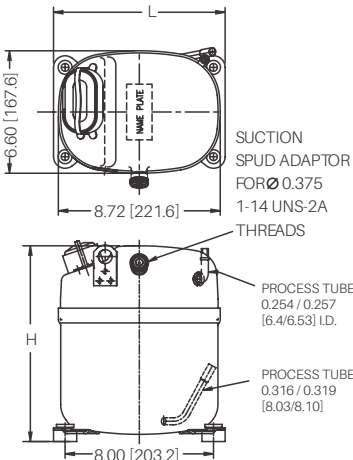
KCJ***CAL with suction tube
