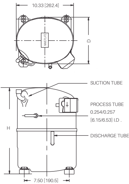
KCM522CAL with Suction Tube
