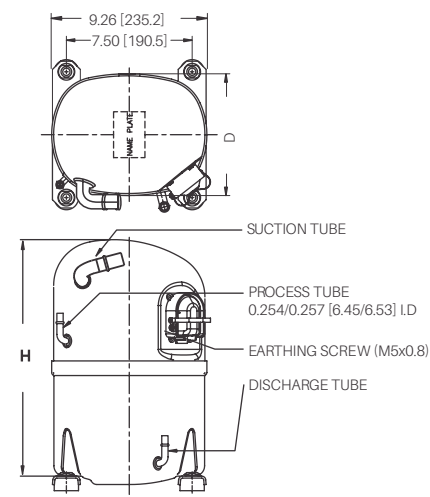
KCM475LAL/KCM511CAL/514CAL with Suction Tube
