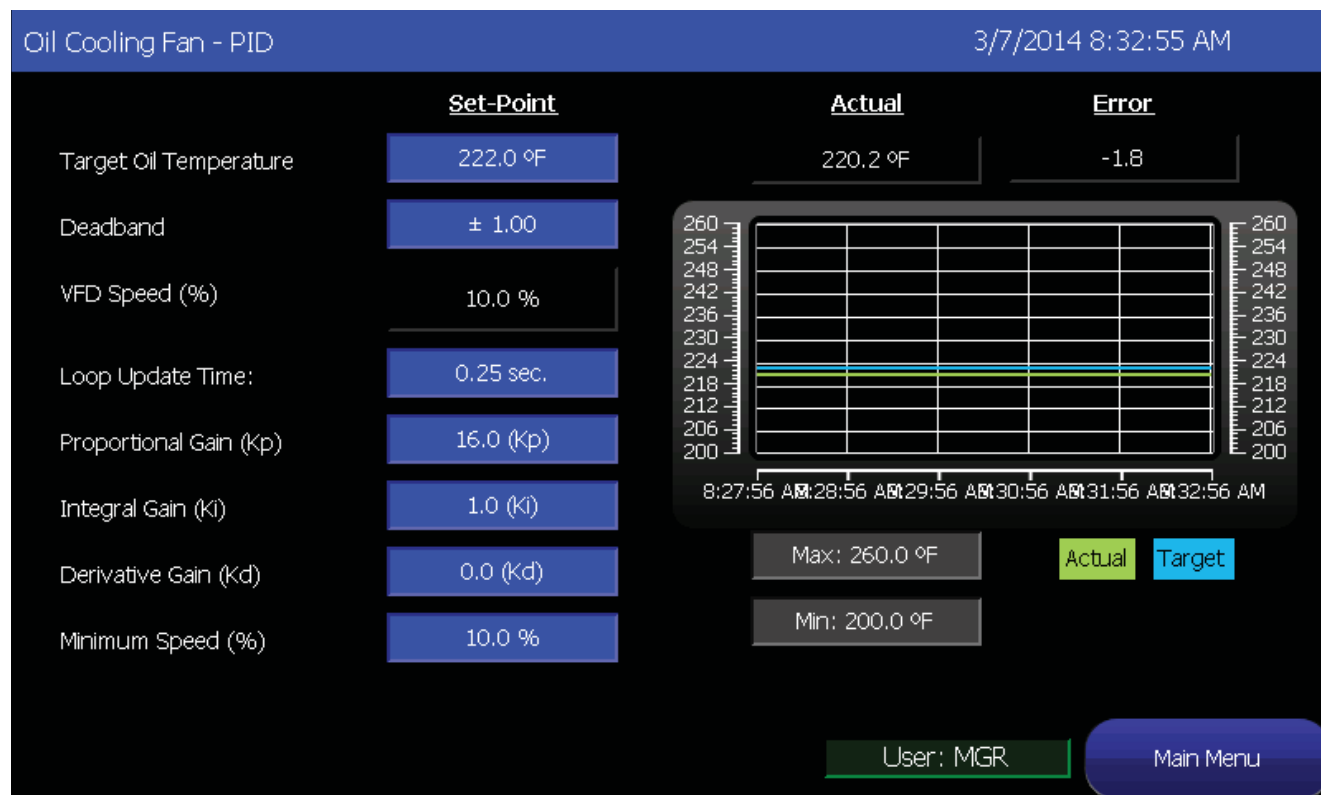
Figure 3-8. Oil Cooling Fan - PID Screen
