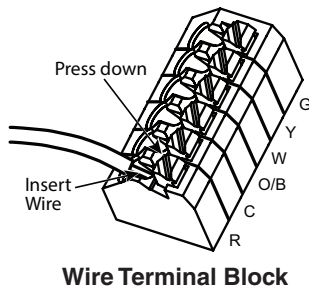
Wire Terminal Block
