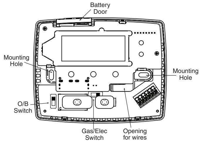
Figure 1. Thermostat Base
