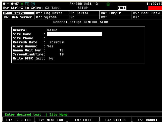
Figure 1 - General Controller Info Setup Screen
